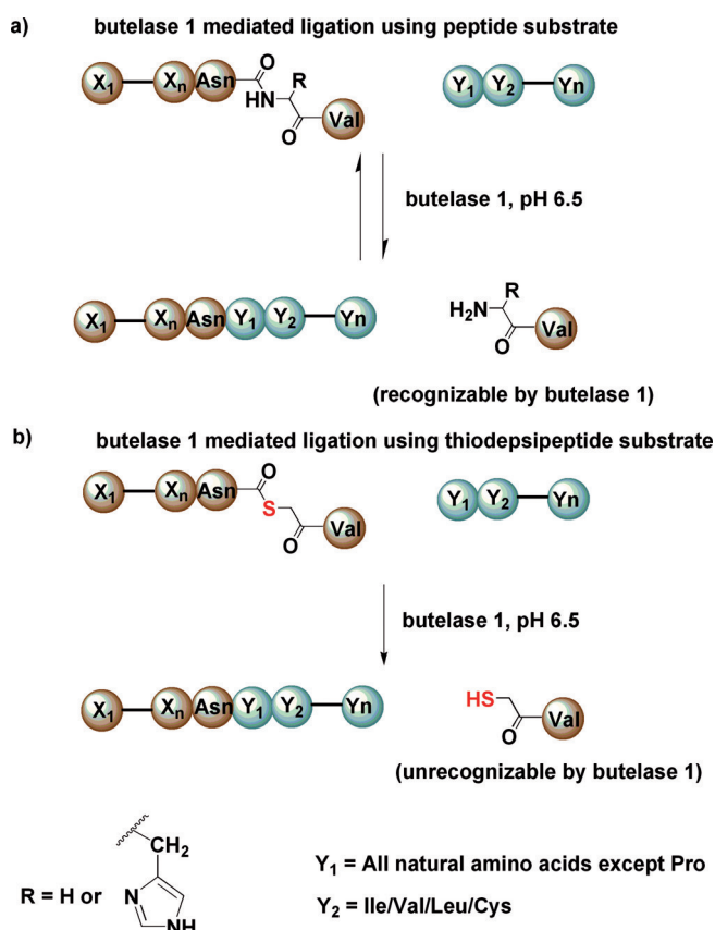
Scheme 1. Butelase 1 ligation using a) natural peptide and b) thiodepsipeptide.
