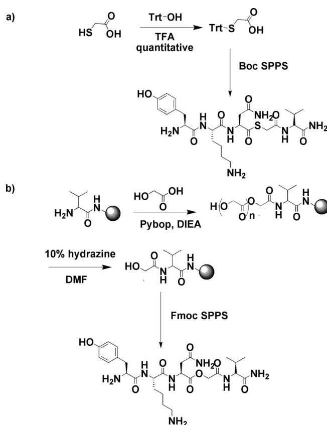
Scheme 2. Synthetic strategy for a) thiodepsipeptide 1 and b) depsipeptide 2 .
